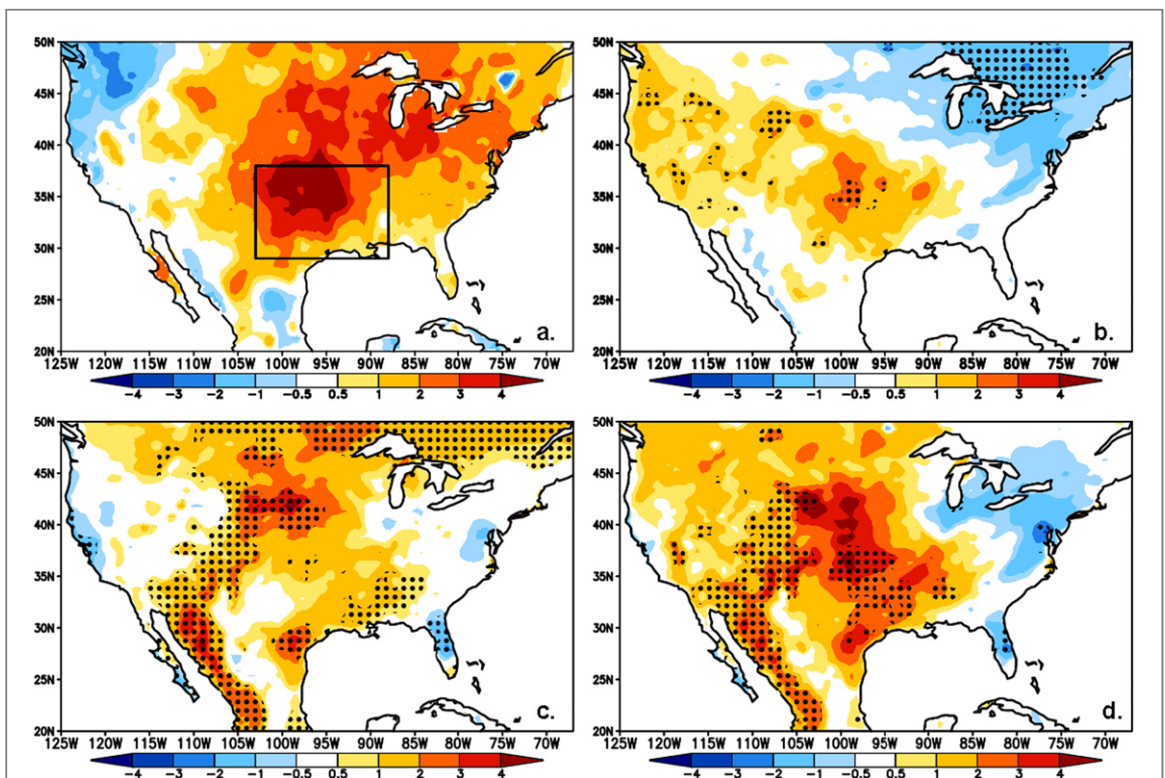
Figure 5. Observed/WRF simulated anomaly/difference of surface temperature ( ^{\circ}\text{C} ) for July. (a) Observed, (b) SUBT effect, (c) SST effect, and (d) SST effect plus SUBT effect. The dotted areas denote statistical significance at the \alpha = 0.01 level of t-test values.
