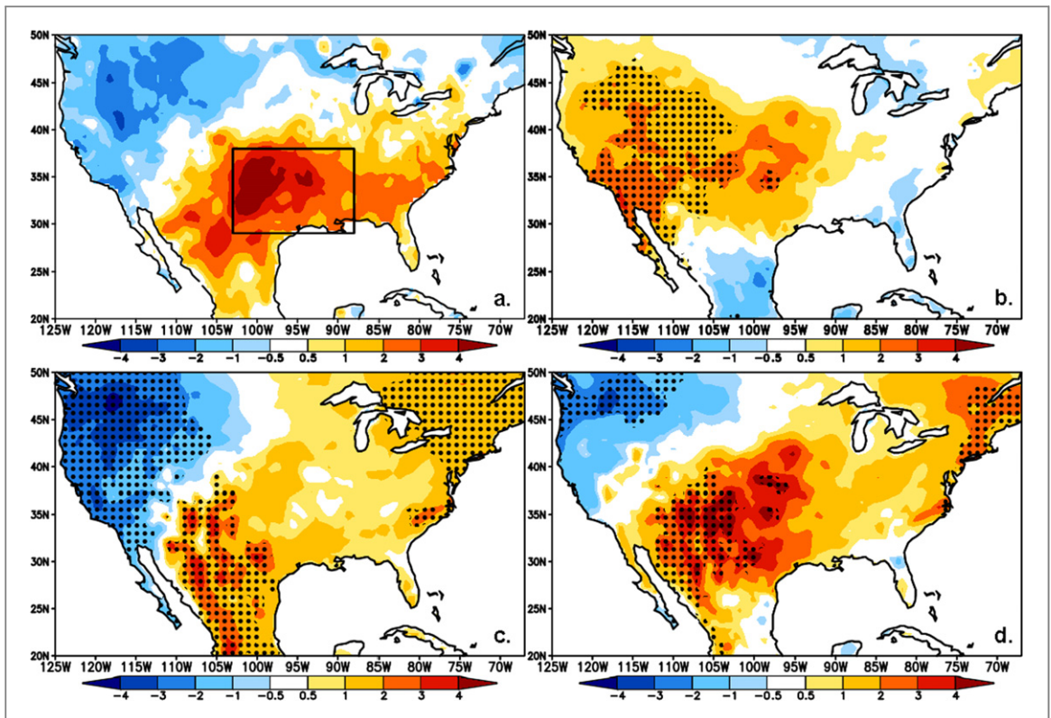
Figure 4. Observed/WRF simulated anomaly/difference of surface temperature ( ^{\circ}\text{C} ) for June. (a) Observed, (b) SUBT effect, (c) SST effect, and (d) SST effect plus SUBT effect. The dotted areas denote statistical significance at the \alpha = 0.01 level of t-test values.
