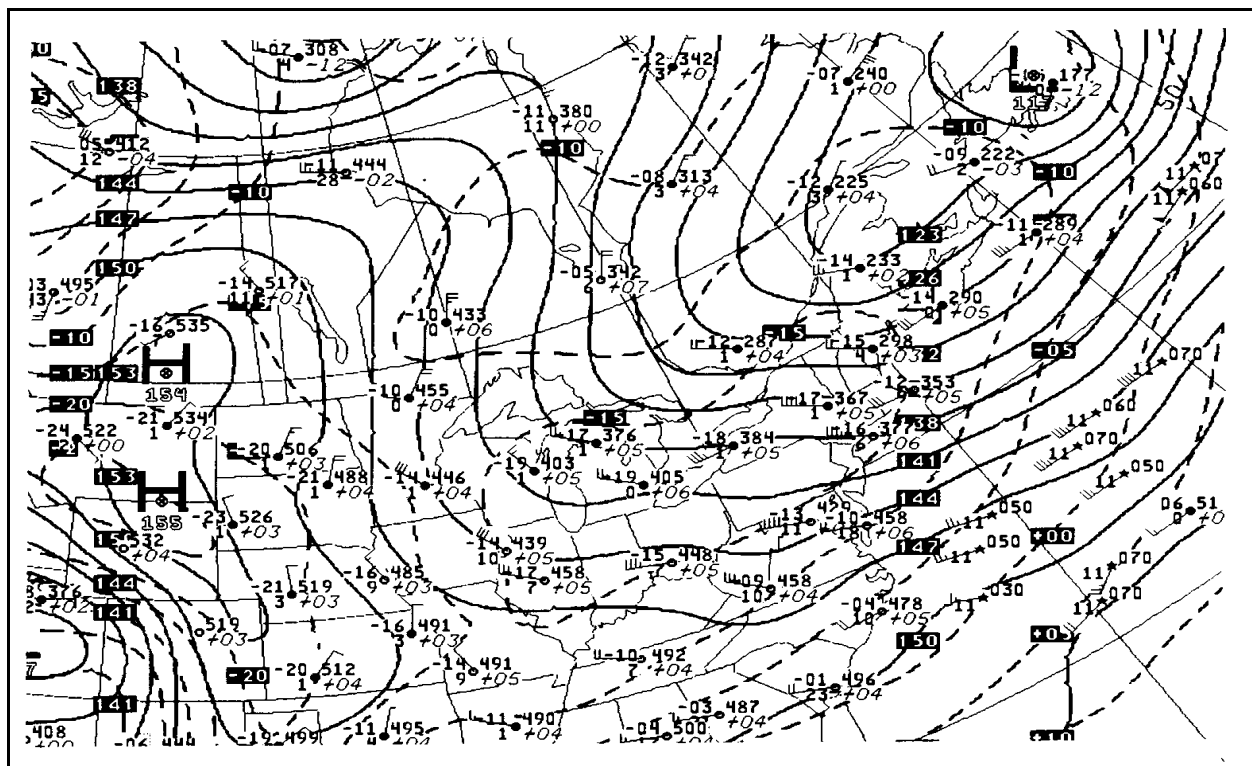
Figure 3: 850-Millibar Temperature, Wind, and Height Analysis for Tug Hill Area at 12:00 UTC on January 12, 1997.
