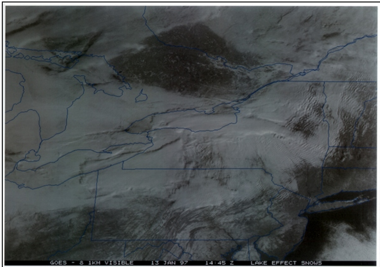
Figure 5: Visible GOES-8 Satellite Image at 9:45 EST on January 13, 1997, Showing a Lake Ontario Snow Plume Streaming Over Tug Hill (and Montague).
