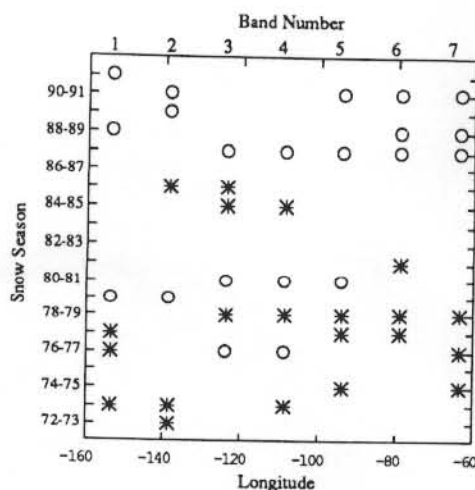
Figure 5. North American Maximum (*) and minimum (O) three snow cover seasons by longitude.
