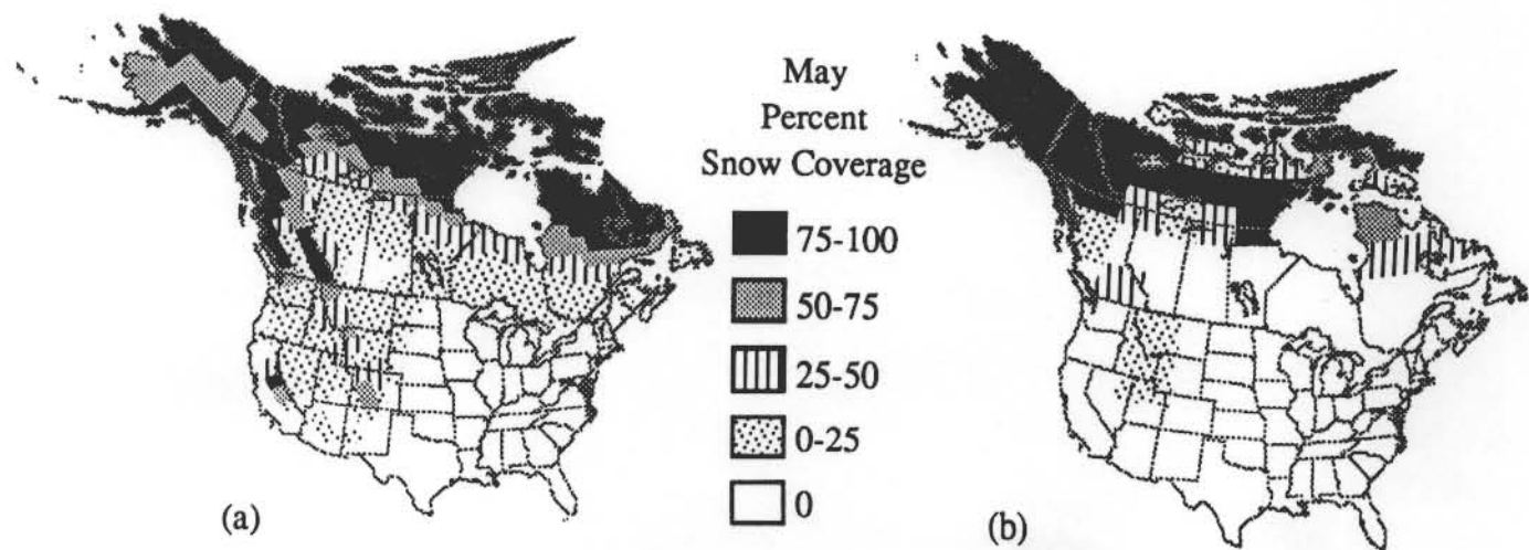
Figure 8. North American percent snow coverage for May (a) from visible imagery 1972-1992, (b) from GFDL GCM results, 10 year control run.
