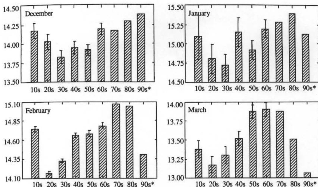
Figure 8. Decadal fluctuations of North American snow cover extent (millions of square kilometers) since the 1910s. The error term for the estimates 1910-1970 are based on differences between station-derived and satellite snow cover within the satellite era, using station distributions from earlier decades. *1990-1996 Jan., Feb., Mar.; 1990-1995 Dec.
