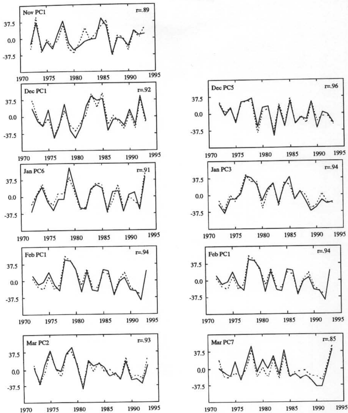
Figure 3. Comparison between observed and modeled regional snow cover extent anomalies (%), 1972-1993. Eastern active region in November is north of the United States border. Solid line=observed extent; dotted line=modeled extent.
