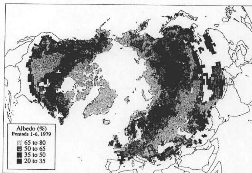
Fig. 1. Estimated surface albedo (in per cent) over snow-covered lands during the first six pentads of 1979. Any 1 \times 1^\circ cell that was snow covered during at least one pentad of this interval is assigned an albedo by averaging the cell values for the six pentads. Snow data are from the NOAA visible snow charts.
