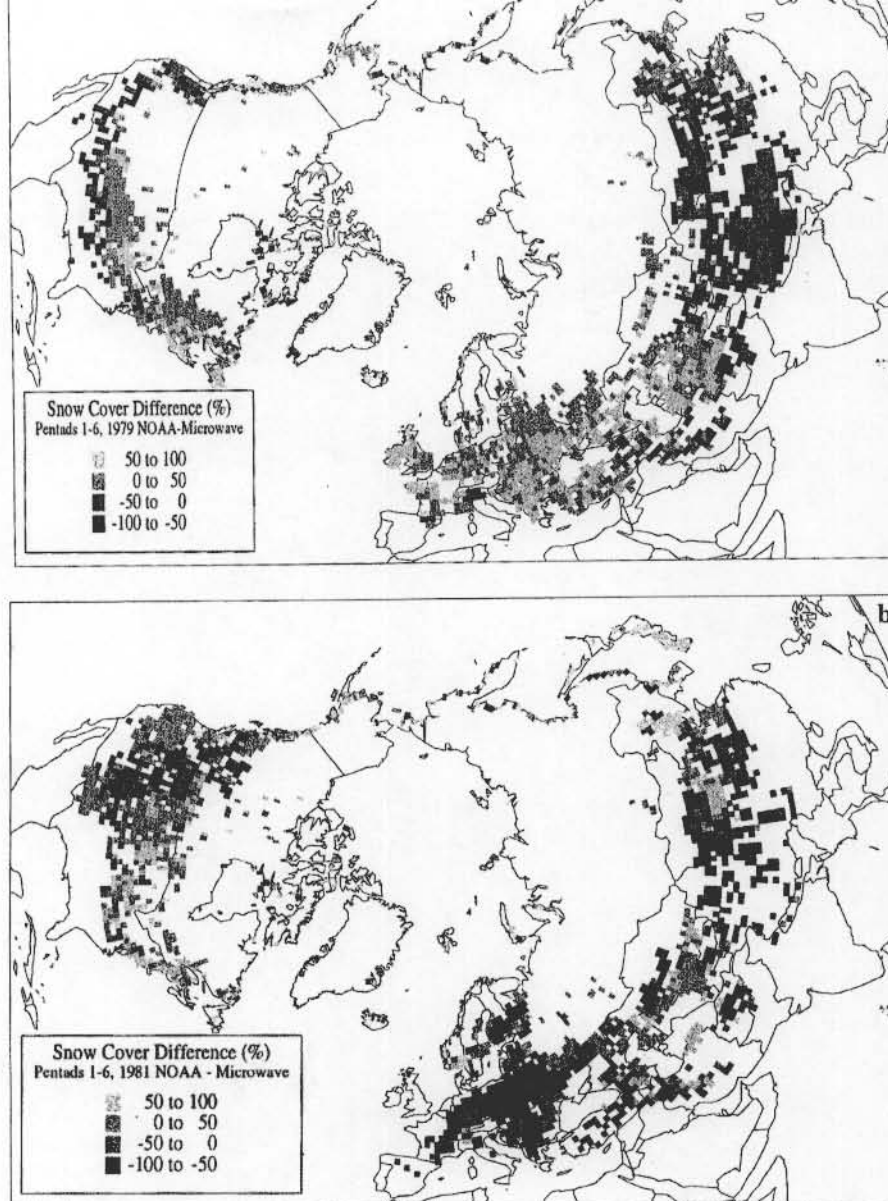
Fig. 3. Difference of visible and microwave snow cover frequencies for the first six pentads of (a) 1979 and (b) 1981. Values are positive (negative) where the visible file shows more frequent cover than the microwave (SMMR) file.
