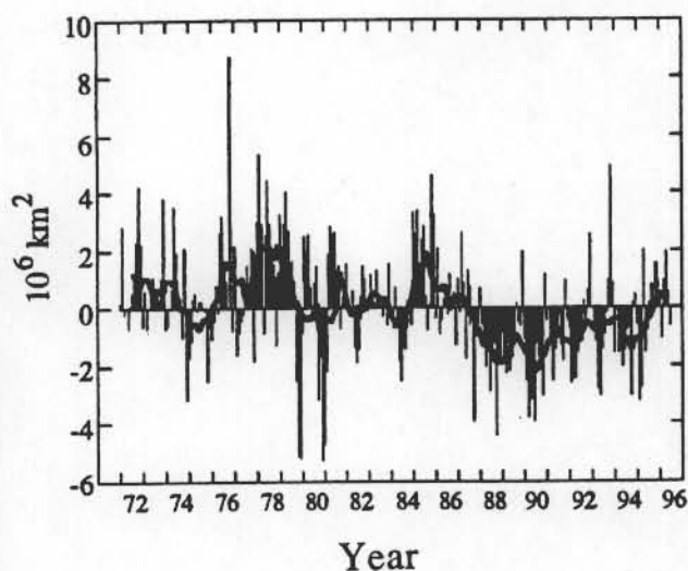
Fig. 4. Anomalies of monthly snow-cover extent over Northern Hemisphere lands (including Greenland) between January 1972 and August 1996. Also shown are 12 month running anomalies of hemispheric snow extent, plotted on the seventh month of a given interval. Anomalies are calculated from NOAA visible charts. Mean hemispheric snow extent is 25.3 \times 10^6 \text{ km}^2 for the full period of record (see Robinson, (1993a) for a discussion of the Rutgers method used to calculate monthly snow cover).
