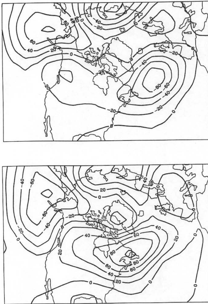
Figure 3. Composite averaged 500-mb height departures (in meters) for Februaries with positive (top) and negative (bottom) snow cover extremes at 45-50°N and 100-105°W. Positive snow years include 1972,75,78,79,82; negative years 1977,81,83,84 (1992 is the fifth negative year, however 500-mb data are as yet unavailable).
