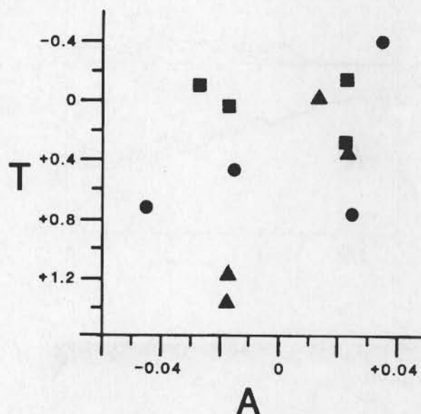
Fig.4. Comparison of monthly anomalies of surface albedo over the Arctic Basin and surface air temperature from 65-85°N for May (triangles), June (circles) and July (squares) of the four study years. Albedo anomalies from the average of the four years. Temperature anomalies based on 1951-1970 means (Jones 1985; Climate Monitor 1985a, 1985b).
